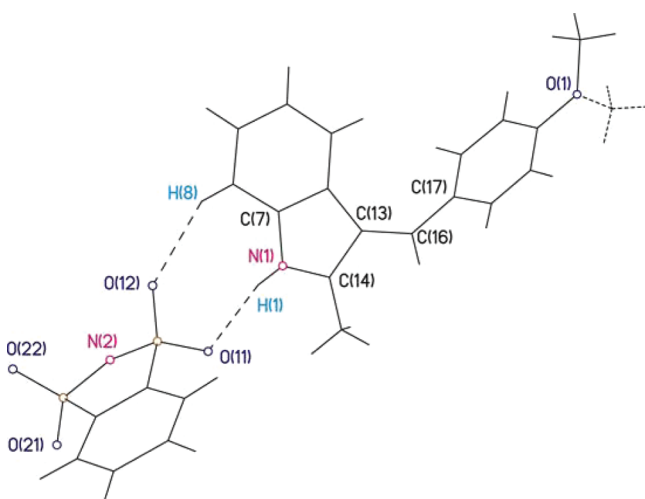
Figure 2. Anion and cation of salt 4b [C 6 H 4 NO 4 S 2 ][C 17 H 16 NO]. Relevant bond lengths (Å) with e.s.d.'s: S(1)–O(12) 1.4348(15), S(1)–O(11) 1.4386(15), S(1)–N(2) 1.555(2), S(2)–O(21) 1.4189(17), S(2)–O(22) 1.4193(17), S(2)–N(2) 1.583(2), N(1)–C(14) 1.306(3), N(1)–C(7) 1.404(3), C(13)–C(16) 1.358(3), C(13)–C(14) 1.447(3), C(16)–C(17) 1.440(3). Methyls attached to O(1) are disordered.
