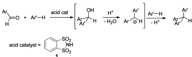
Scheme 3. Triarylmethane Synthesis Catalyzed by o -Benzenedisulfonamide ( 1 )
