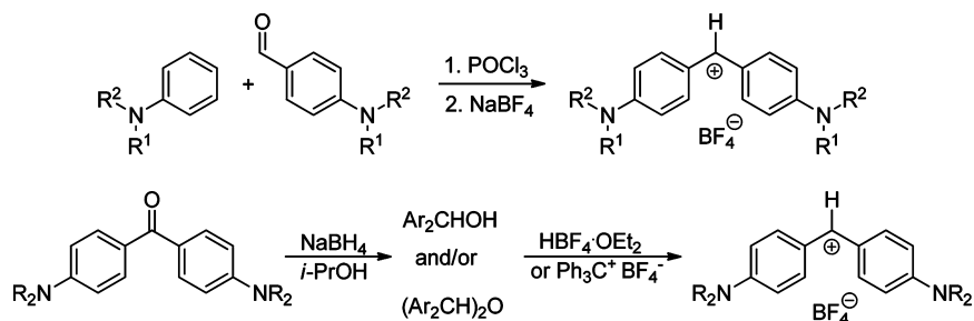
Scheme 1. Benzhydrylium Tetrafluoroborate Syntheses
