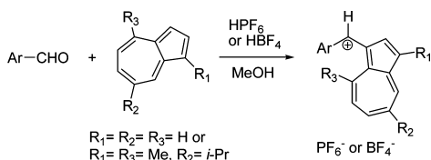
Scheme 2. Syntheses of Carbenium Salts Stabilized by a 1-Azulenyl or a 3-(Guaiazulenyl) Group
