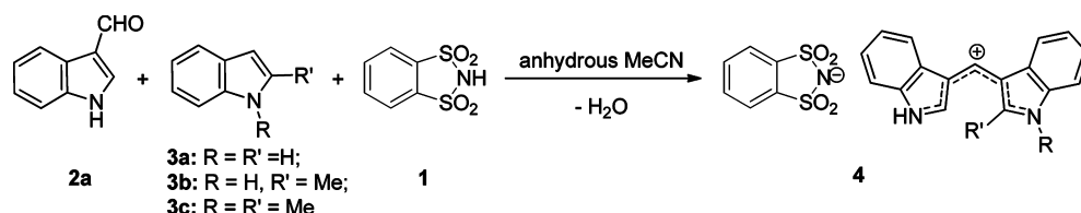
Scheme 4. Synthesis of o -Benzenedisulfonimide Salts 4 Starting from 3-Formylindole
