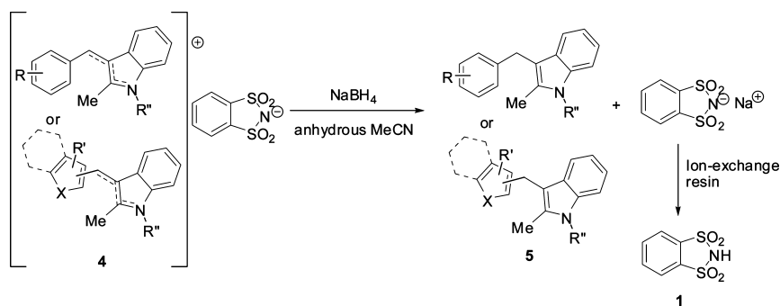
Scheme 5. Reduction of Salts 4 to Diarylmethanes 5
